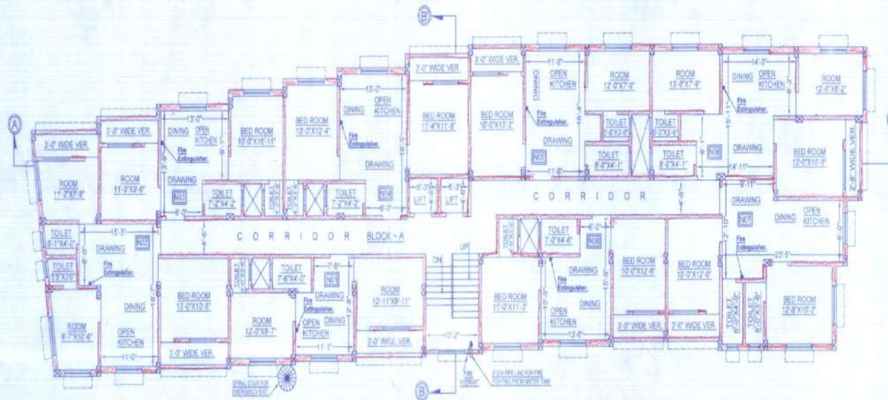
PROPOSED TYPICAL FLOOR PLAN ( 2ND, 3RD, 4TH. & 5TH.) (BLOCK - A)
