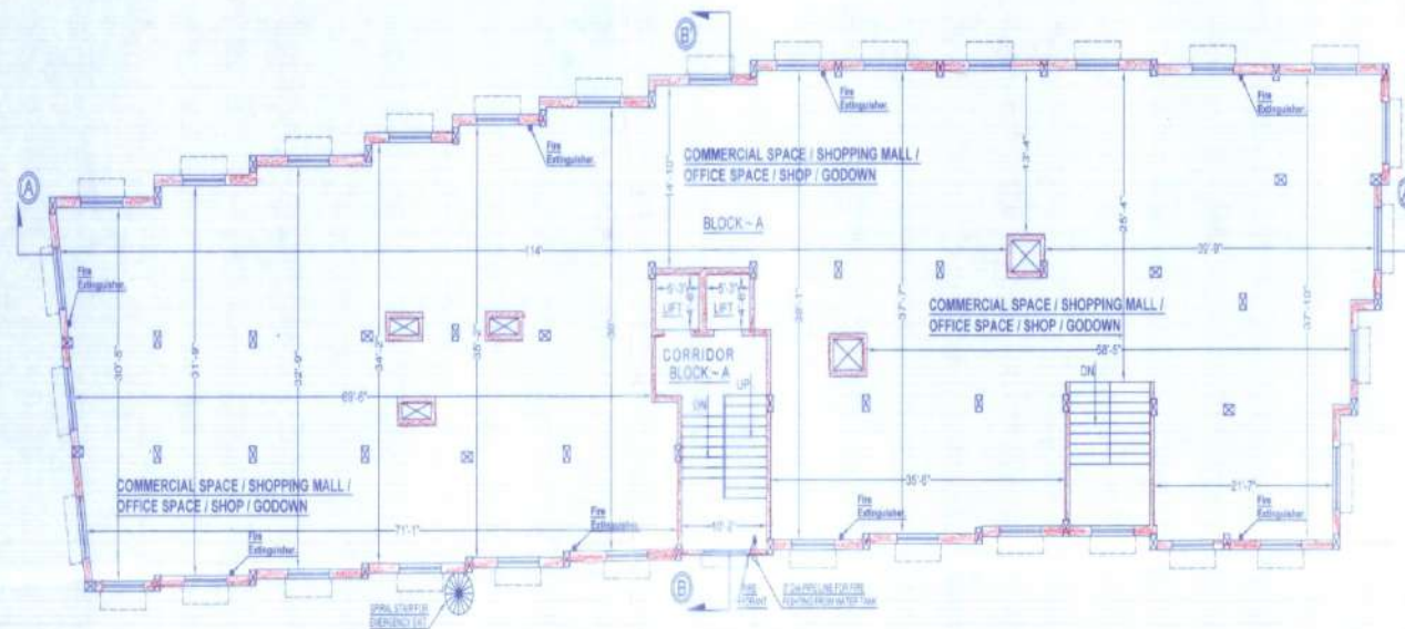
PROPOSED FIRST FLOOR PLAN (BLOCK - A)
