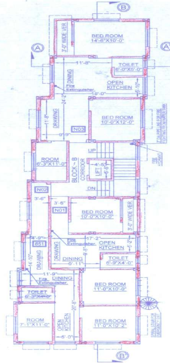
PROPOSED TYPICAL FLOOR PLAN (1ST., 2ND, 3RD., 4TH. & 5TH.) (BLOCK - B)
