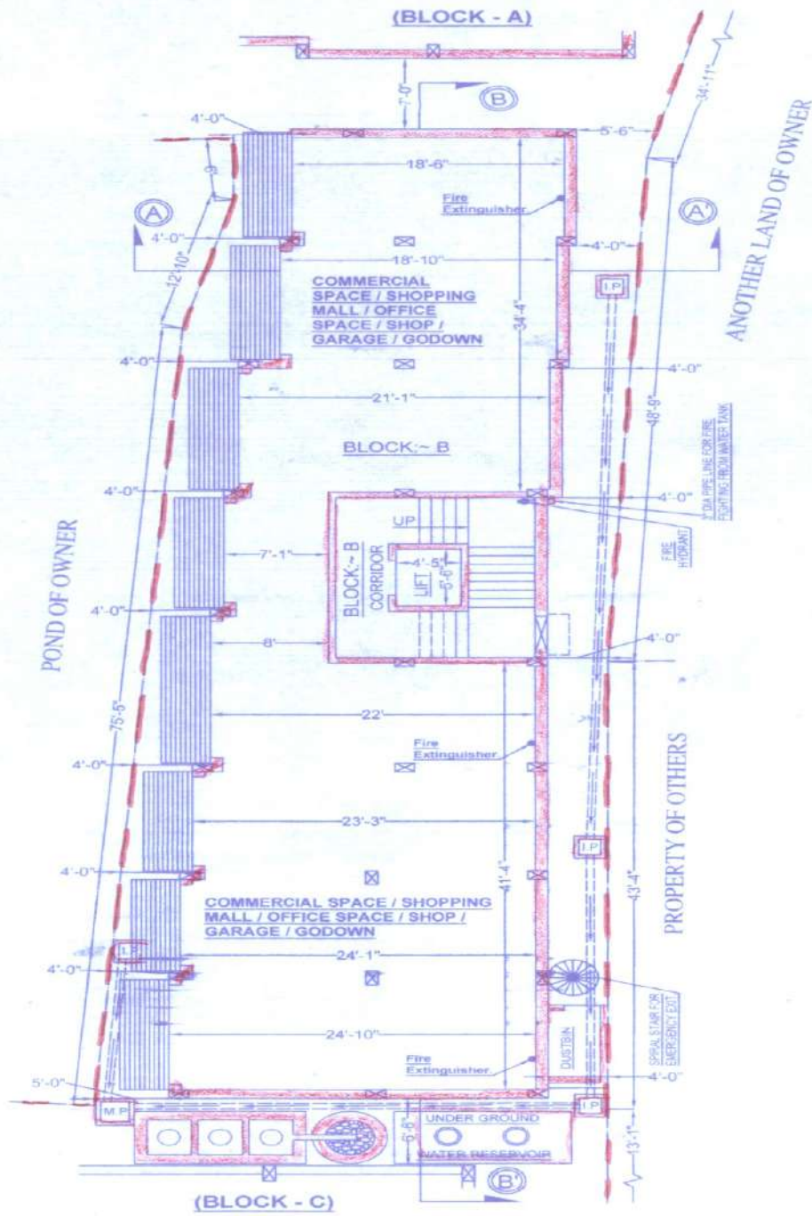
PROPOSED GROUND FLOOR PLAN (BLOCK - B)
