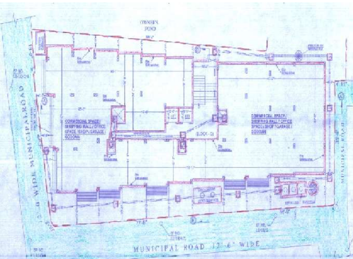
PROPOSED GROUND FLOOR PLAN (BLOCK - C)
